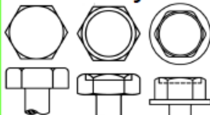
Trimmed Hex Indented Hex Hex Washer
